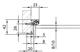
Profilquerschnitt | Profile sectional cut
